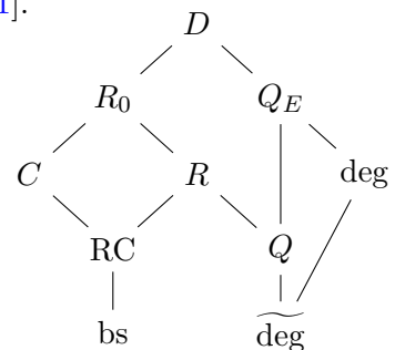
Figure 2: Relations between complexity measures.
