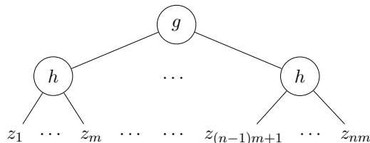
Figure 1: Composed function g \circ h .
