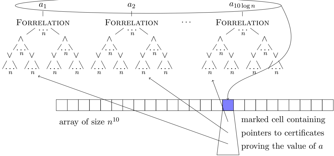
Figure 3: The function f that achieves a superquadratic separation between Q(f) = \tilde{O}(n) and R(f) = \tilde{\Omega}(n^{2.5}) .
