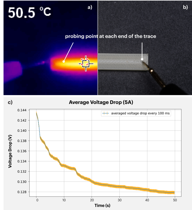
Figure 9: Trace conductivity and current capacity test sample: a) and b) the exterior temperature stabilizes at approximately 50^\circ \text{C} under a 5 A current load; c) the EGaIn trace voltage drop measured over 50 s under a 5 A current.
